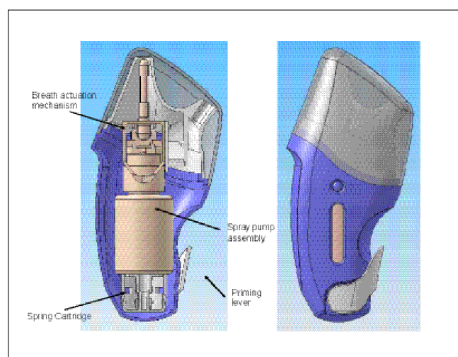
Figure 1. Breath-actuated bi-directional delivery device. The basic functional components are shown, along with the styled exterior (15) .
